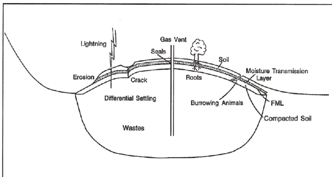
Figure 2 Factors Affecting Landfill Cover Integrity
